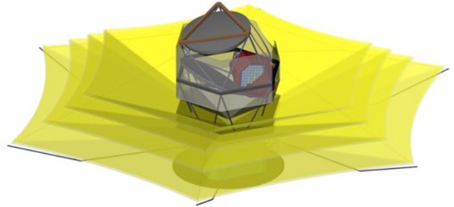
Figure 3: The EPIC-IM mission observes the CMB sky with a 1.4 m off-axis telescope and a large focal plane of bolometric detector arrays operating at 100 mK. The telescope is cooled to 4 K, first through 4 fixed V-groove radiators to 25 K, and then by a pulse-tube refrigerator. A deployed 15-m sun shield is used to keep solar radiation from heating the optics. An 18 K radiation shield surrounding the telescope has been removed to show the optics and focal plane.
