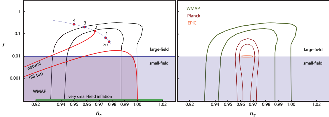
Figure 2: Left Panel: Predictions of single-field slow-roll models in the n_s - r plane. The figure shows the WMAP 5-year constraints on n_s and r (68% and 95% confidence levels in black) as well as the predictions of a few representative models of single-field slow-roll inflation: chaotic inflation \lambda_p \phi^p , for general p (thin solid line) and for p = 4, 3, 2, 1, \frac{2}{3} (red dots); natural inflation and hill-top inflation (red solid lines); and very small-field inflation (green bar). Right Panel: Same WMAP constraints as on the left together with projected 68% and 95% constraints from Planck and the proposed EPIC-IM space-based mission assuming r = 0.01 and n_s = 0.965 . The EPIC-IM prediction includes errors due to the subtraction of simulated foregrounds.
