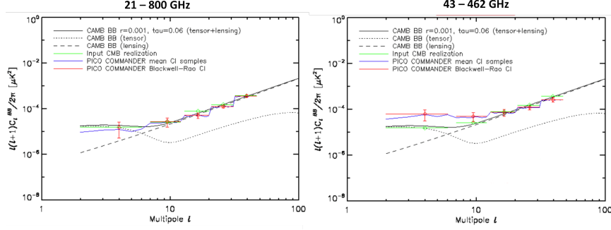
Figure 16: Foreground removal with all of PICO’s 21 frequency bands (left panel) recovers the input CMB (green) without any bias (red) using the Commander algorithm on the Planck sky model (with 4 deg pixels, and 50% sky fraction). Running the same algorithm on the same sky without several of the lowest and highest bands (right panel) produces an output spectrum (red) that is biased relative to the input (green) at low \ell multipoles. The bias would be interpreted as higher value of r relative to the model input (solid black) with r = 0.001 (dots) and lensing (dash).
