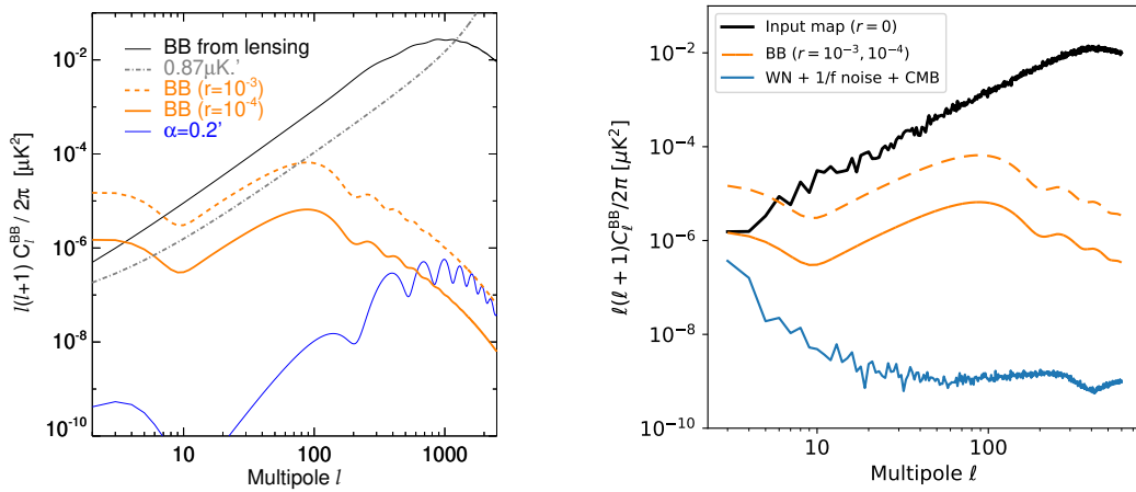
Figure 2.17: Two of the initially-estimated highest priority systematic effects for PICO can be suppressed to low levels relative to requirements; we show inflationary signals with r = 1 \times 10^{-4} and 1 \times 10^{-3} (solid and dash orange, respectively), and BB lensing (black, theory on the left; realization on right). Left: The residual spurious BB spectrum due to 0.2' mis-calibration of PICO’s angles of polarization sensitivity (solid blue) has the shape of the EE spectrum, and is small compared to the requirement for \ell < 200 and compared to the baseline statistical noise level (grey dash). Right: simulated residual BB power after accounting for calibration drifts (solid blue).
