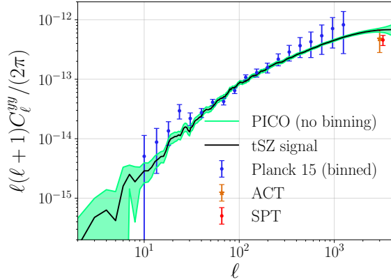
Figure 2.10: The PICO y-map will give a tSZ power spectrum with an SNR of 1270 (green, 1\sigma per \ell mode), which is nearly 100 times larger than from Planck (blue). Binning the data (not shown), as was done for Planck would further increase the SNR. We also show current measurements by the ground-based SPT and ACT [128, 129]. In these forecasts we reconstruct the Compton-y field from maps that include Galactic foregrounds, CMB fluctuations, and PICO CBE noise using the needlet internal linear combination algorithm [130]. The input maps use the Planck sky model [131].
