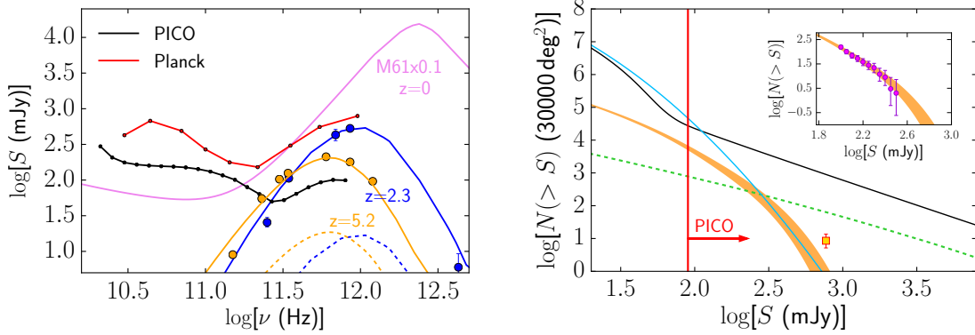
Figure 2.13: Left: PICO will detect thousands of new strongly lensed galaxies near the peak of their spectral energy distributions (SEDs), such as SMM J2133–0102 (blue) at z = 2.3 [189] and HLS J091828.6+514223 (orange) at z = 5.2 [190]. The dashed lines are the SEDs before magnification by lensing. PICO’s higher resolution gives point-source detection limits (black line) that are up to 10 times fainter than Planck ’s 90% completeness limits (red line [191]). High-frequency measurements ( \nu > 300 GHz) of 30,000 low- z galaxies, like M61 (magenta, SED was scaled down by a factor of ten), will give a census of their cold dust. Right: Integral counts of unlensed (black) and strongly lensed, high- z (orange) star-forming galaxies for 70% of the sky away from the Galactic plane at 600 GHz based on fits of Herschel counts over 1000 \text{deg}^2 (inset [186]). The PICO detection region (right of vertical red line) will yield a factor of 1000 increase in strongly lensed galaxies relative to Planck (yellow square), as well as about 50,000 proto-clusters (blue) and 2,000 radio sources (green) [192].
