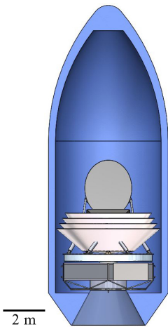
Figure 4.1: PICO is compatible with the Falcon 9.
