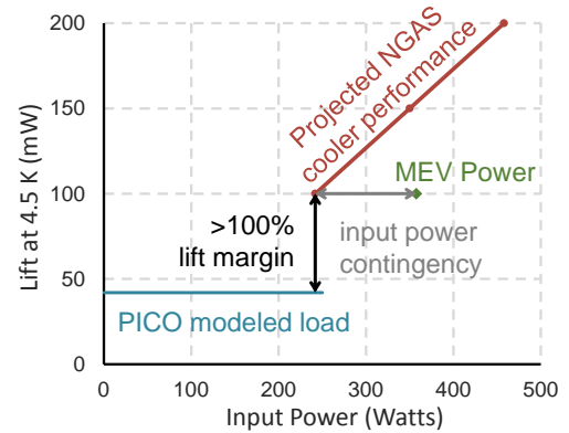
Figure 3.4: Projected performance of the NGAS cooler using a multi-stage compressor and ^4\text{He} circulating gas [283] meets PICO’s requirements with > 100 % margin. PICO requires heat lift of 42 mW at 4.5 K (Table 3.3). With 250 W of input power the NGAS cooler is projected to provide 100 mW of heat lift. We conservatively specify a maximum expected value (MEV) of 350 W as the compressor’s input power, giving 100 W of additional input power contingency.
