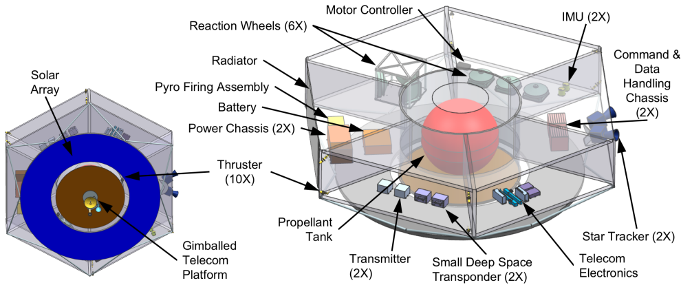
Figure 4.3: Modular equipment bays provide easy access to all components in the spacecraft de-spun module and enable parallel integration of spacecraft subsystems.
