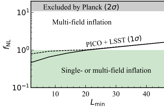
Figure 2.3: Cross-correlating PICO’s lensing potential map with LSST galaxies will allow detecting or excluding f_{\text{NL}}^{\text{local}} = 2 with 3\sigma evidence if the data can be used at angular scales L \geq 8 (solid black). A detection above |f_{\text{NL}}^{\text{local}}| = 1 indicates that inflation is driven by multiple fields; single-field inflation has |f_{\text{NL}}^{\text{local}}| < 1 (green region). The Planck constraint is f_{\text{NL}}^{\text{local}} < 10.8(2\sigma) . The cross-correlations will allow excluding or detecting f_{\text{NL}}^{\text{local}} = 2(2\sigma) if LSST data are used only for L \geq 20 (dash). Fig. 2.8 gives the assumptions used here for the LSST data.
