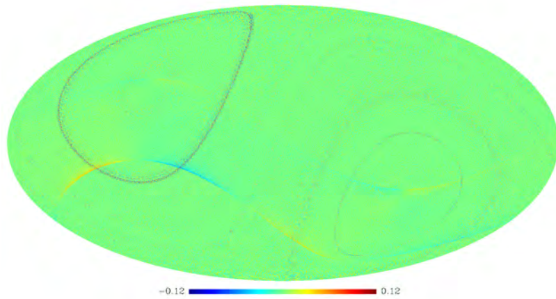
\langle \cos(2\beta) \rangle ; polarization w.r.t. NEP; galactic frame
