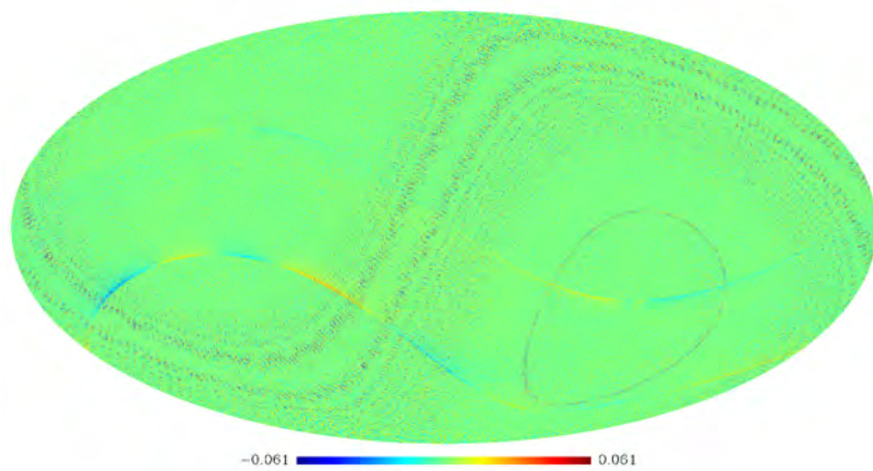
\langle \sin(2\beta)\cos(2\beta) \rangle ; polarization w.r.t. NEP; galactic frame
