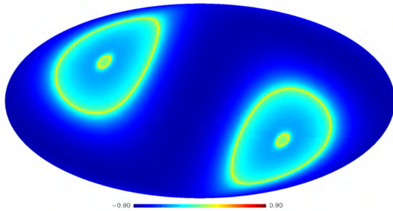
\langle \sin(2\beta) \rangle ; polarization w.r.t. NEP; galactic frame
