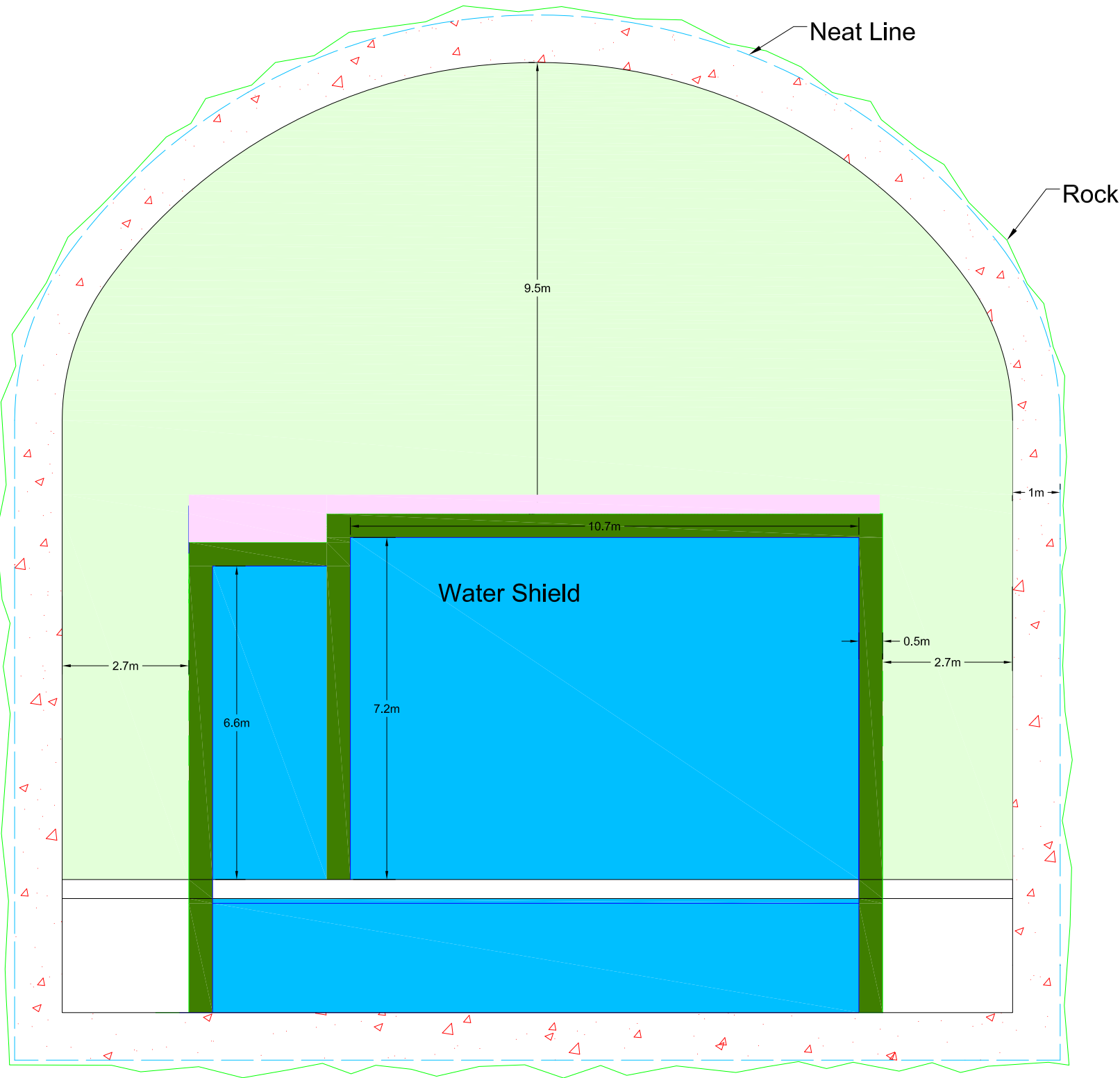
FAARM SECTION CC
