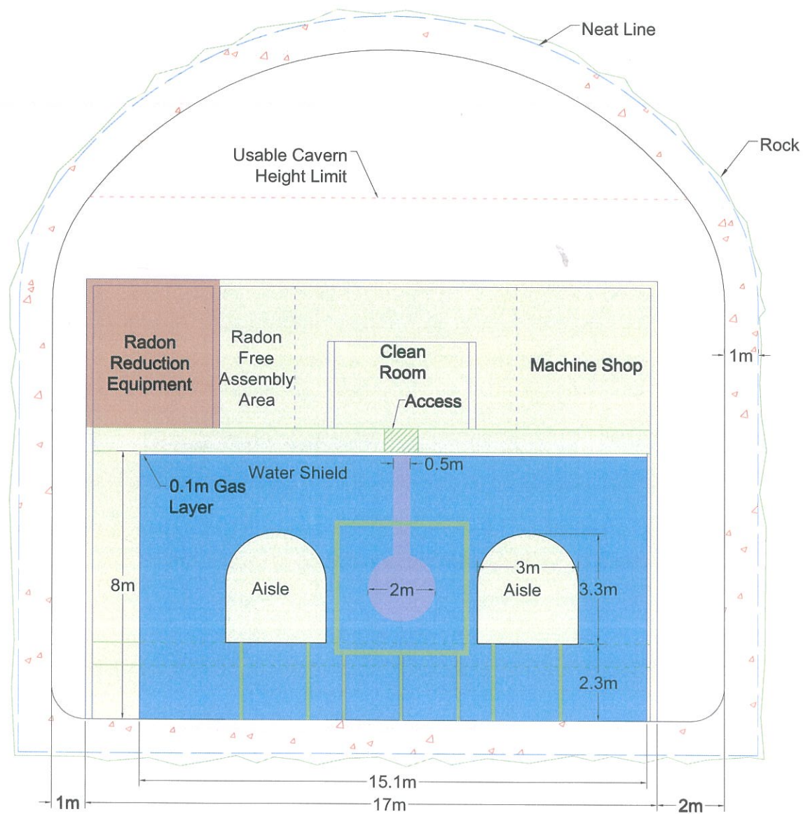
1 GA-04 Water Shield Section 0 2m 4m
