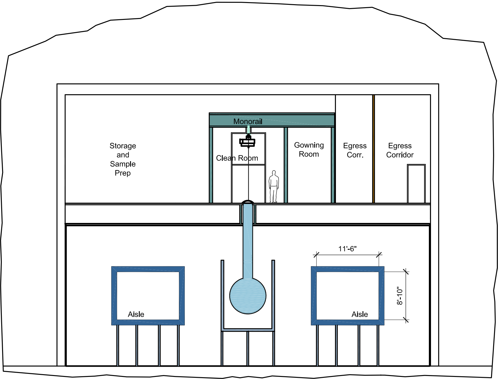
1 A5 FAARM - TANK AREA SECTION - ALTERNATE SECTION THROUGH LARGE CAVERN 3/32" = 1'-0"
