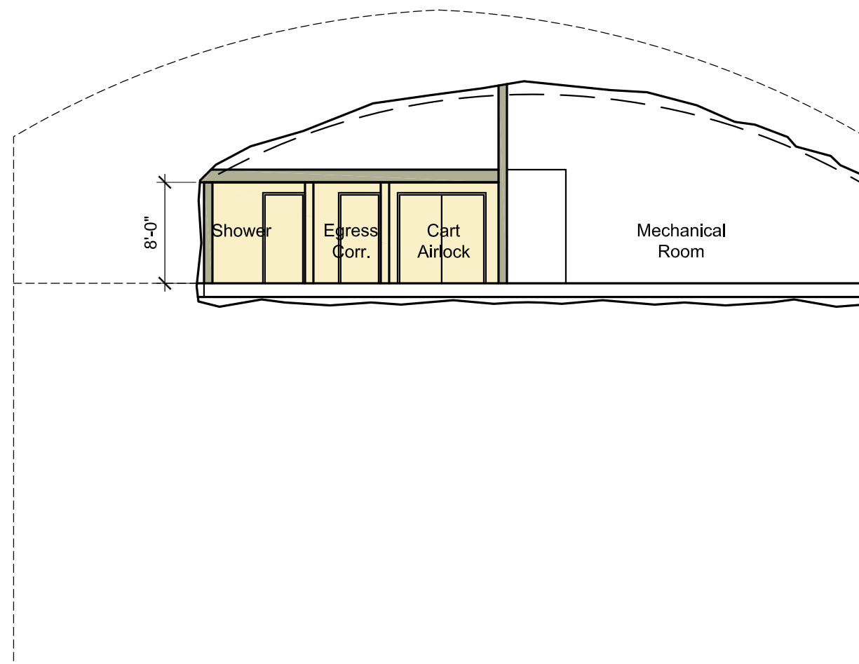
1 FAARM - TRANSITION AREA SECTION A4 3/32" = 1'-0"
