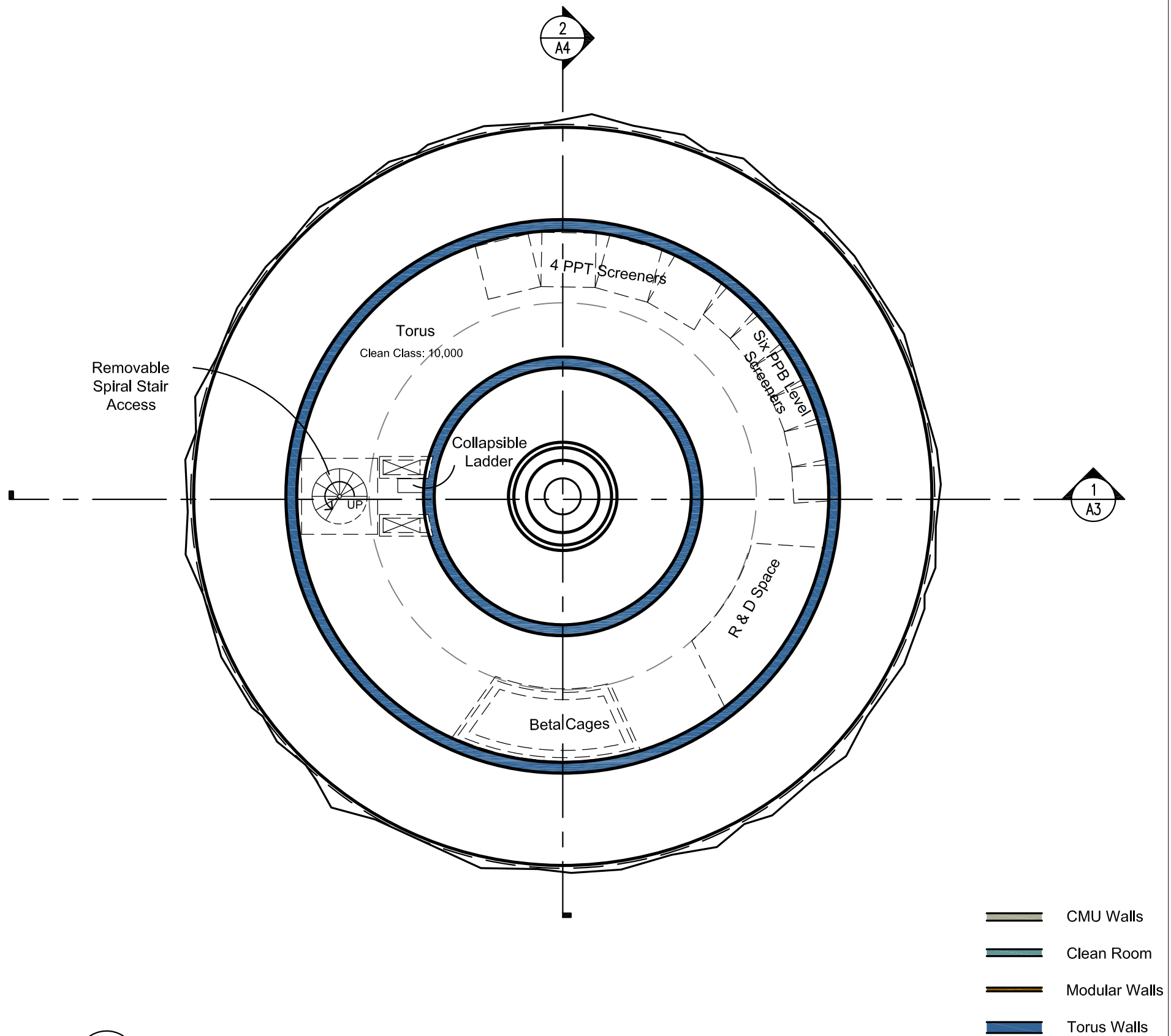
1 A2 FAARM - TORUS FLOOR PLAN 3/32" = 1'-0"
