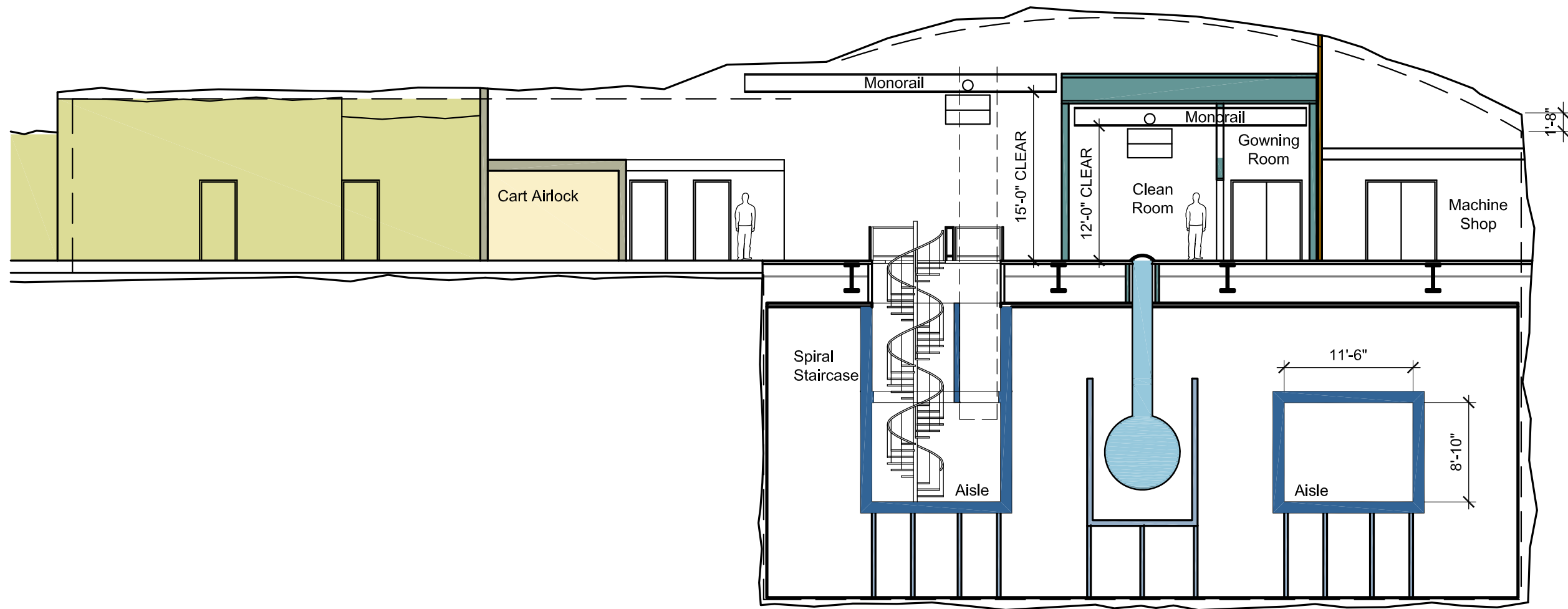
1 FAARM - LONGINTUDINAL SECTION A3 3/32" = 1'-0"
