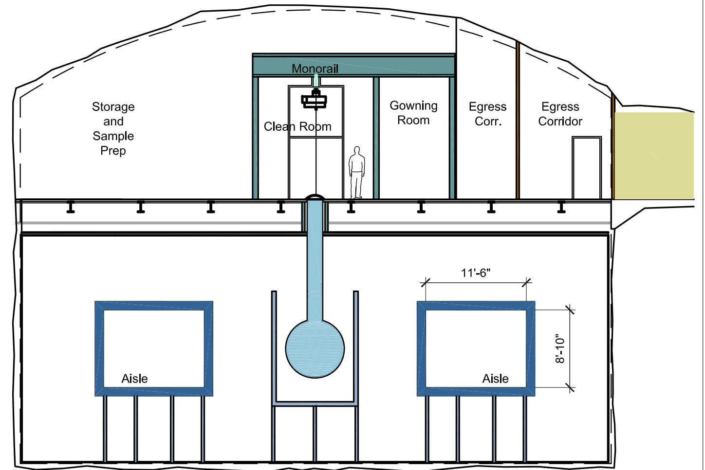
2 FAARM - TANK AREA SECTION A4 3/32" = 1'-0"
