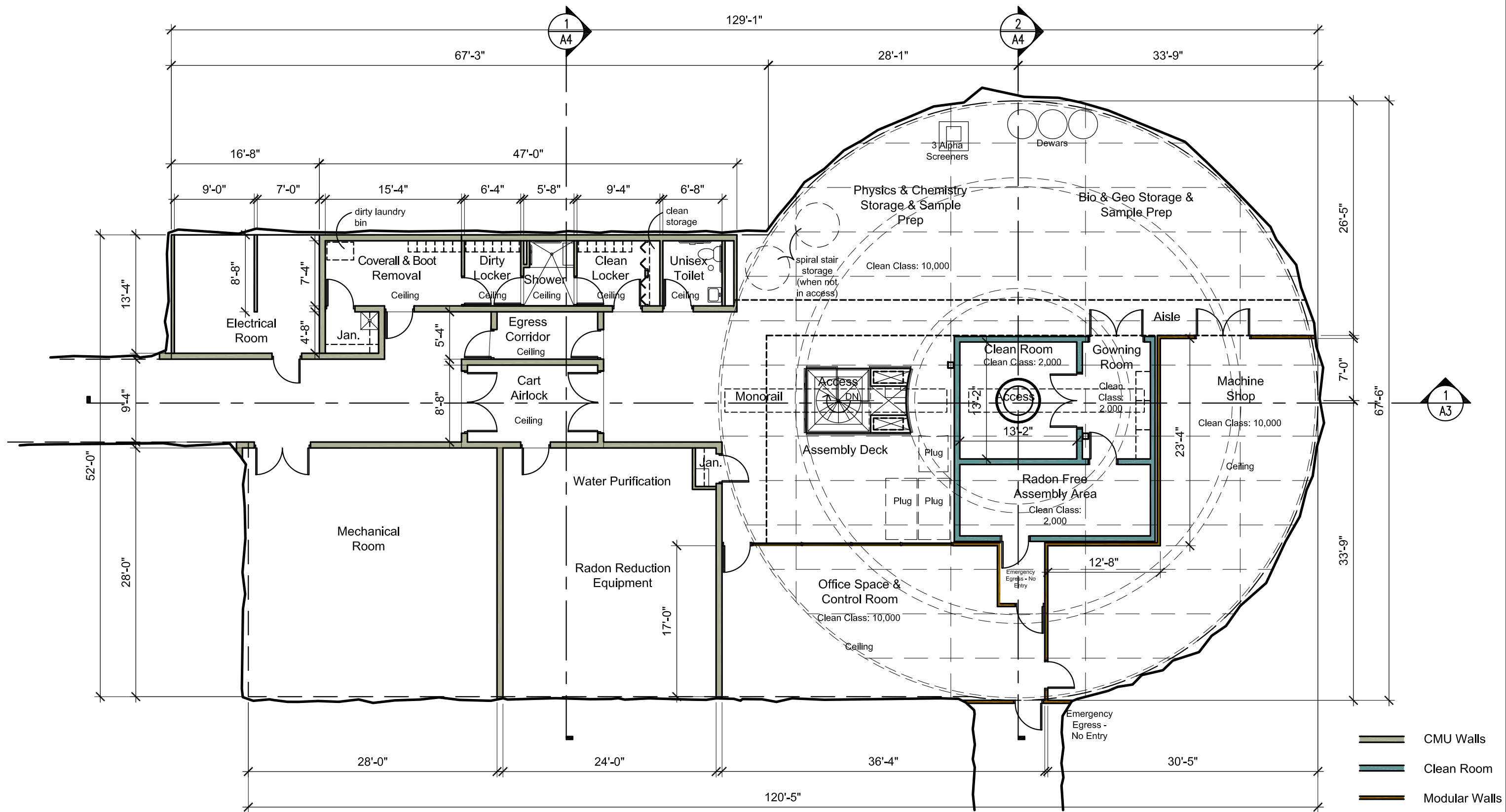
1 FAARM - MAIN FLOOR PLAN A1 3/32" = 1'-0"
