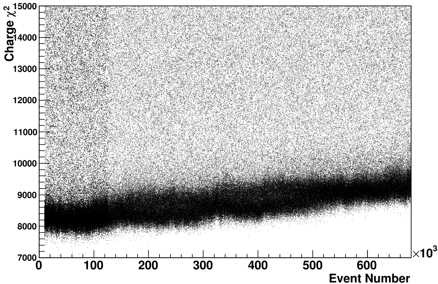
Am-241 Charge \chi^2 vs. Event Number (s)
