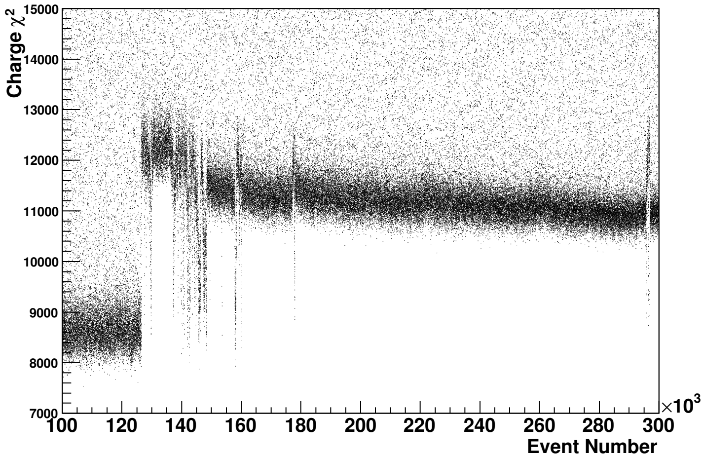
Ba-133 \chi^2 vs. Event Number (s)
