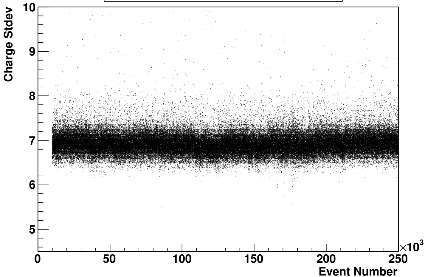
Cf-252 Qlstd vs. Event Number (s)
