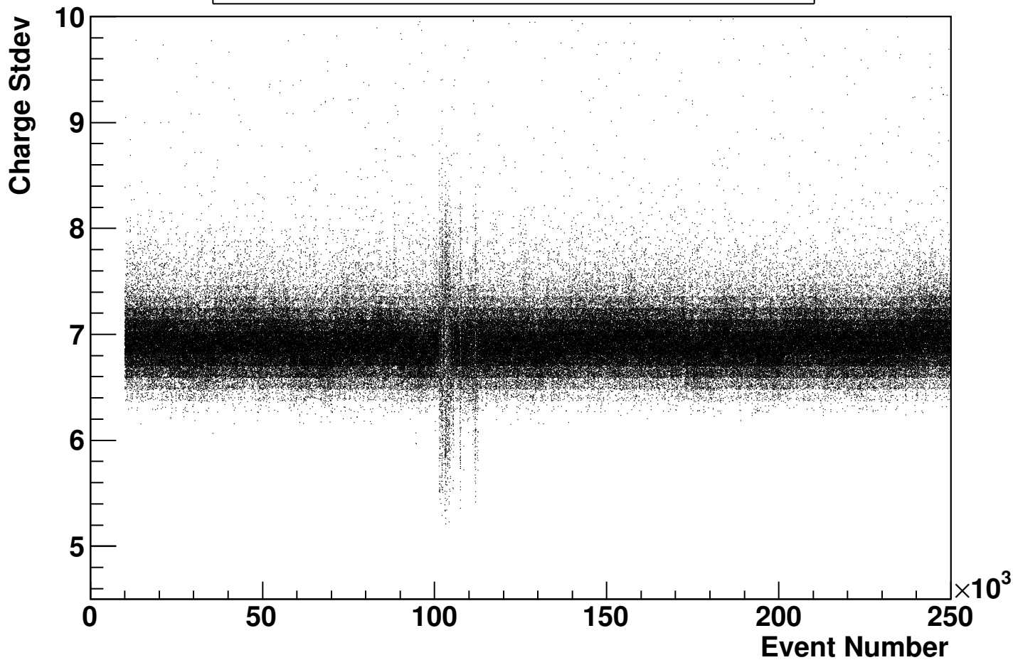
Cf-252 Qlstd vs. Event Number (u-s)
